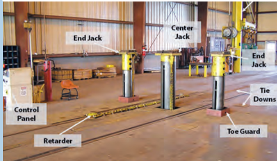
Hydraulic Rail
